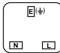
SOCKET (face view)
